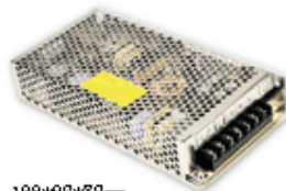
S-120 199*98*38mm
