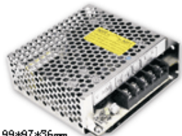
S-15 99*97*36mm
