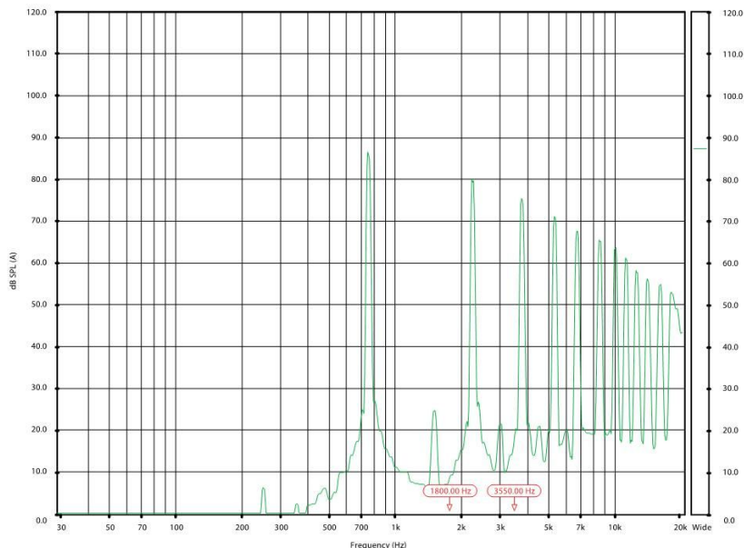
Figure 4 : Fourier analyse square wave 754 Hz
