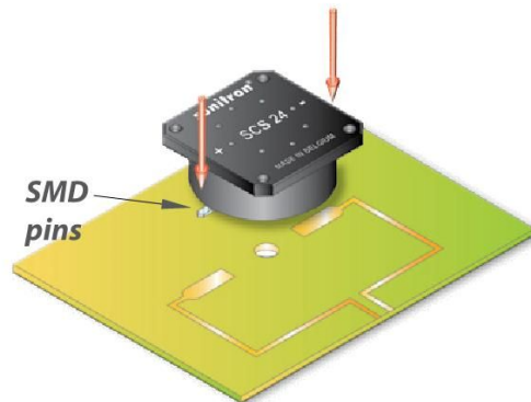
SMD soldered on the PCB
