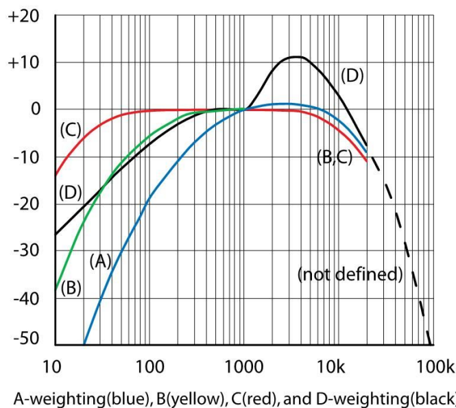
A-weighting curve
