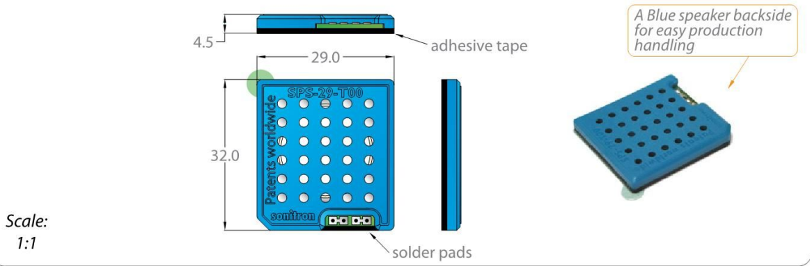
SPS-29-T00
