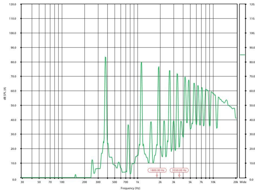
Figure 2: Fourier analyse square wave 374 Hz
