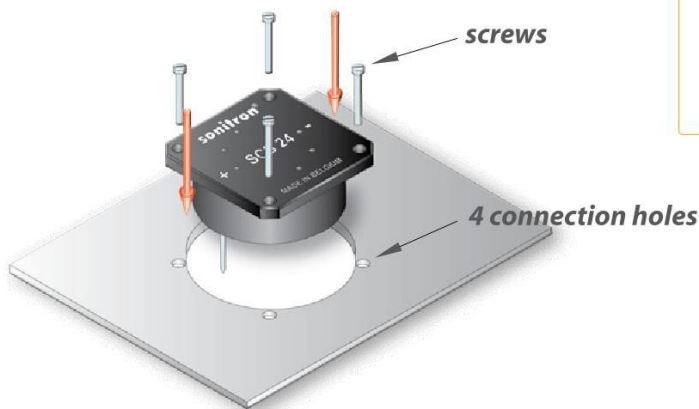
Panel mounting, secured with 4 screws
