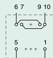
Recommended layout for transformers with 1 secondary winding
